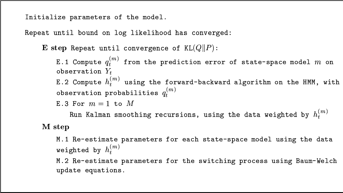
Figure 5: Learning algorithm for switching state-space models.
