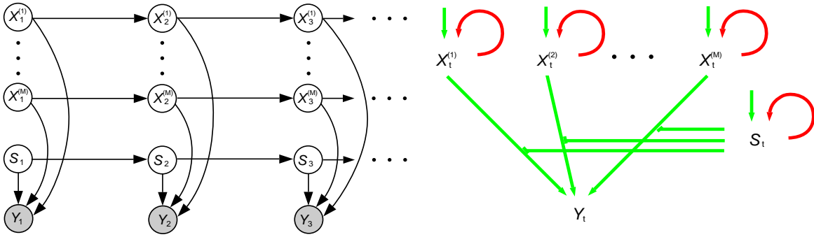
Figure 3: a) Graphical model representation for switching state-space models. S_t is the discrete switch variable and X_t^{(m)} are the real-valued state vectors. b) Switching state-space model depicted as a generalization of the mixture of experts. The light arrows correspond to the connections in a mixture of experts. In a switching state-space model, the states of the experts and of the gating network also depend on their previous states (dark arrows).
